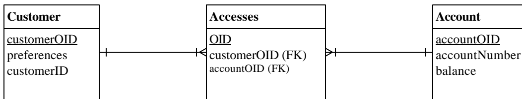
Figure 12. Implementing a many-to-many relationship in a relational database.
