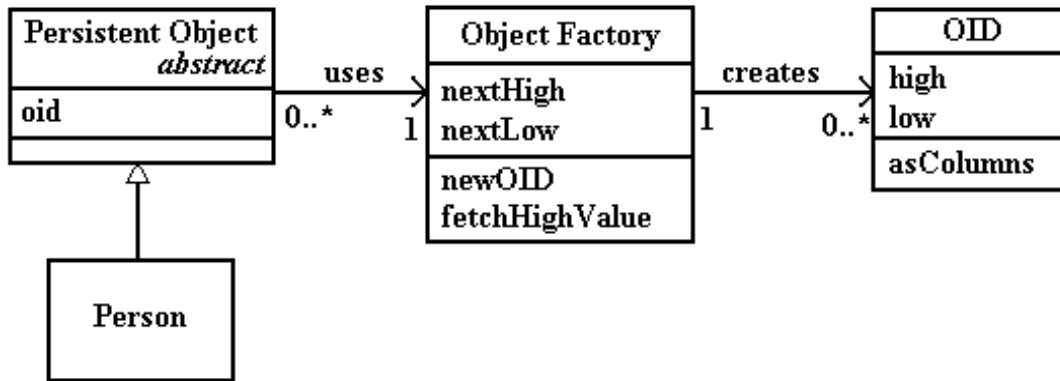
Figure 1. A class diagram showing a possible way to implement a HIGH/LOW OID.
